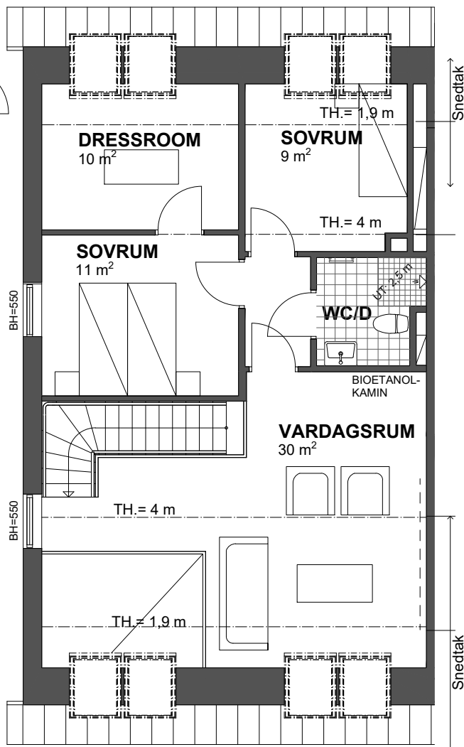
(PLAN 5)
