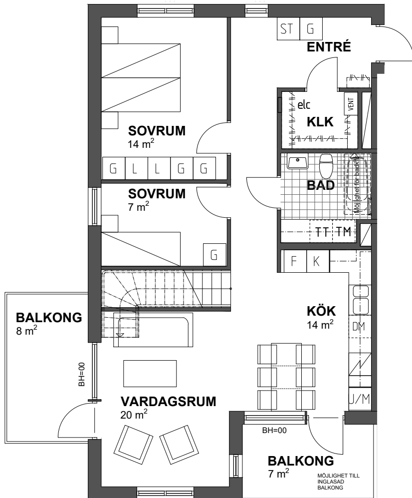
(PLAN 4- 79 m 2 )
