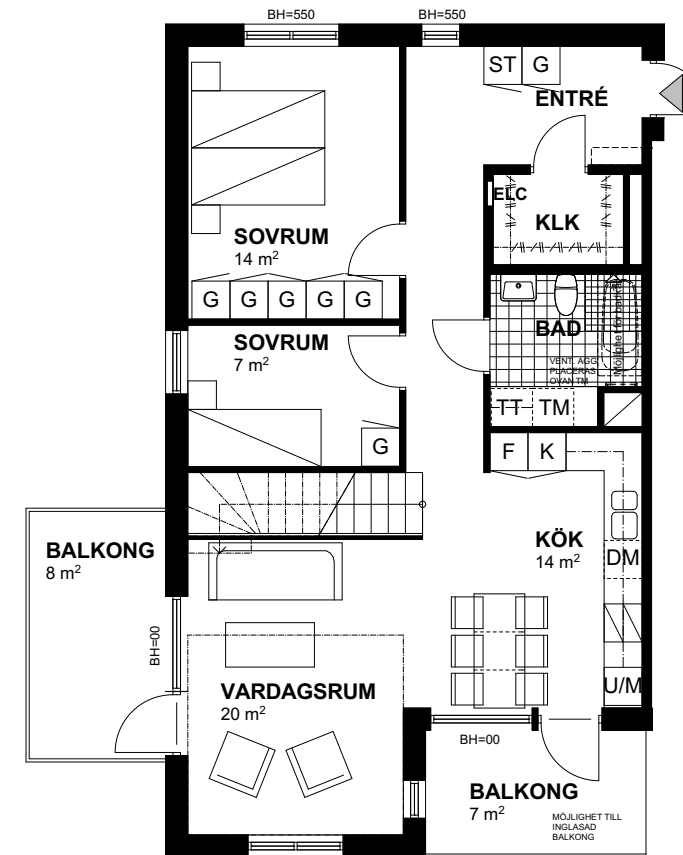
(PLAN 4- 79 m 2 )
