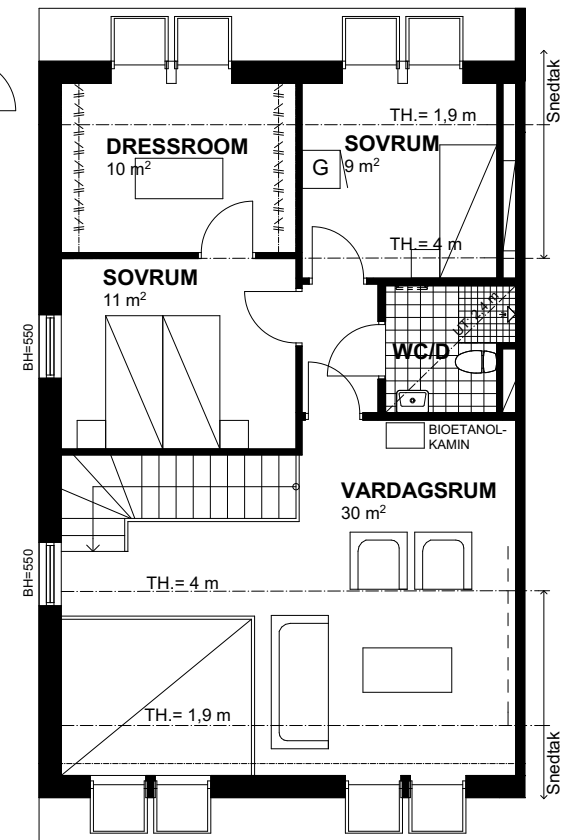
(PLAN 5)
